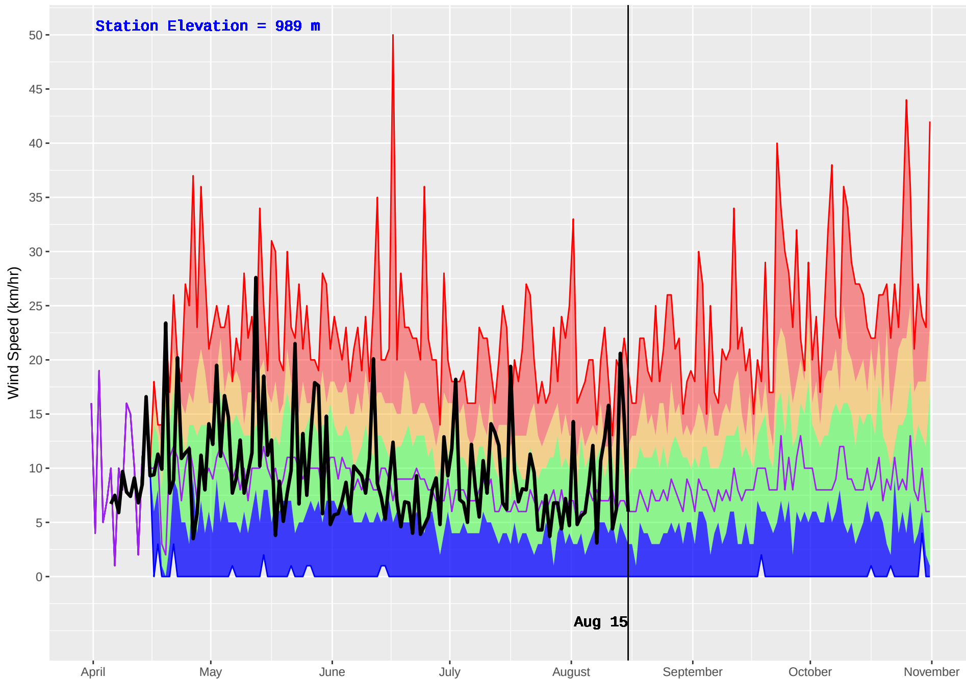
PINK MOUNTAIN (129) : Historical (1983–2016) and Current (2018) Daily Wind Speed
